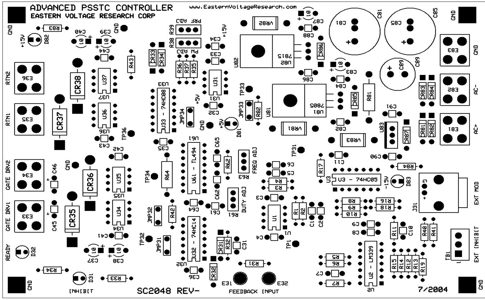
Advanced PSSTC Board - Silkscreen
