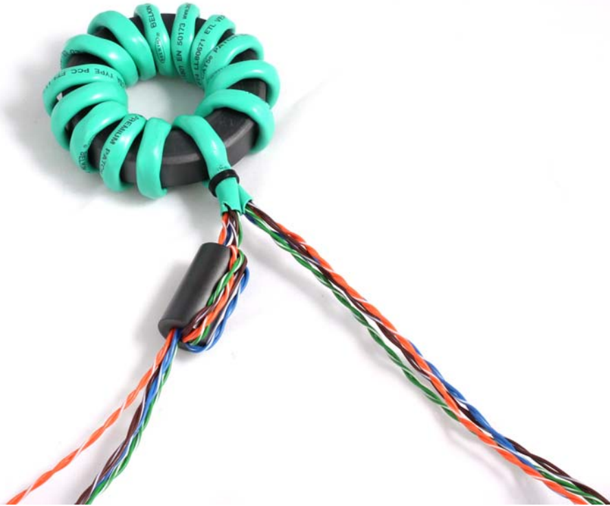
Typical Application – Gate Transformer using flexiBrute Ferrite Toroid Core 5000-1 (shown with flexiBrute Ferrite Suppression Core 31-1)
