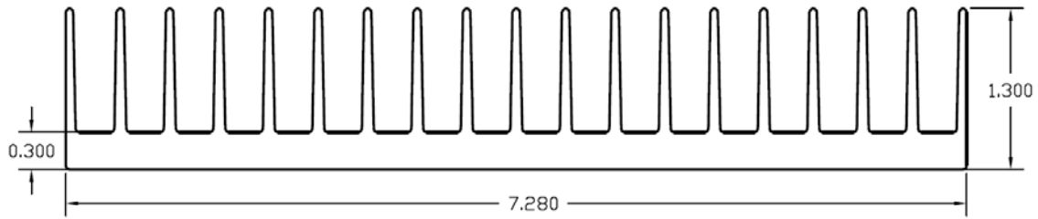
flexiBrute Heatsink 7.3 Profile (Thermal Impedance 1.30 °C/W/3.00")
