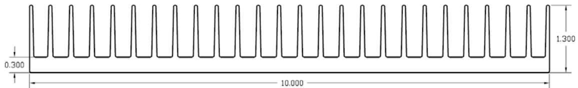
flexiBrute Heatsink 10.0 Profile (Thermal Impedance 0.90 °C/W/3.00")
