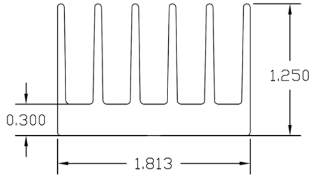
flexiBrute Heatsink 1.8 Profile (Thermal Impedance 4.50 °C/W/3.00")
