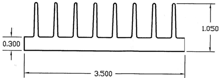
flexiBrute Heatsink 3.5 Profile (Thermal Impedance TBD °C/W/3.00")
