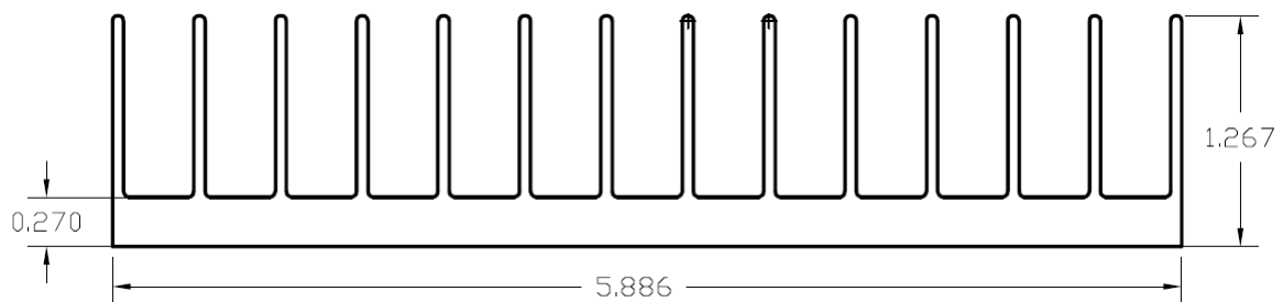
flexiBrute Heatsink 5.9 Profile (Thermal Impedance 1.75 °C/W/3.00")
