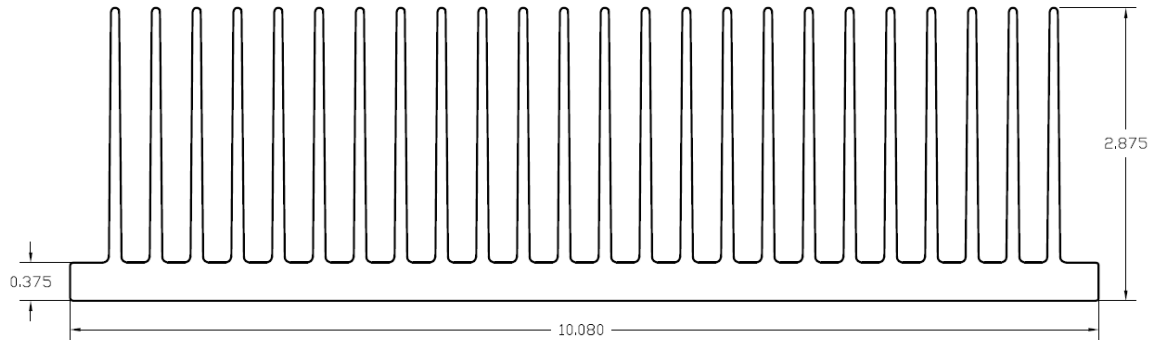
flexiBrute Heatsink Profile 10.1 (Thermal Impedance 0.80 °C/W/3.00")
