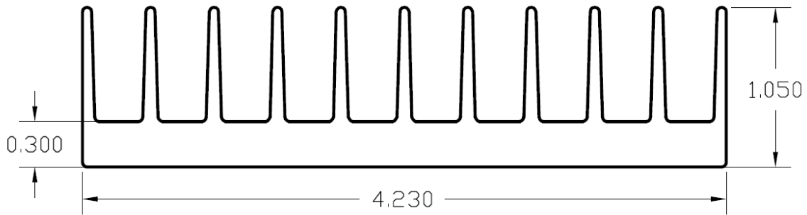
flexiBrute Heatsink 4.2 Profile (Thermal Impedance 2.15 °C/W/3.00")
