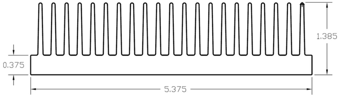
flexiBrute Heatsink 5.4 Profile (Thermal Impedance 1.15 °C/W/3.00")
